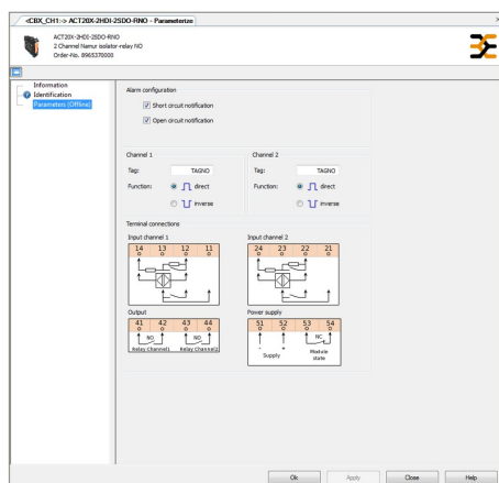
Screenshot of configuration with FDT/DTM software
